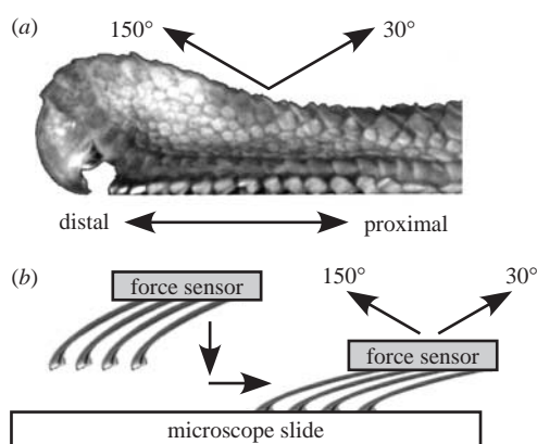
Figure 2. Geometry of isolated setal array detachment tests. (a) Side view of a tokay gecko toe showing the proximal (0°; towards animal) and distal (180°; away from animal) directions. (b) Isolated setal arrays were loaded vertically and then dragged proximally to attach. Once adhering, setal arrays were detached along a linear path of angles ranging from 30° to 150° in increments of 10°. Setal array reaction force and displacement was measured during detachment, yielding work of detachment ( W_d ).
